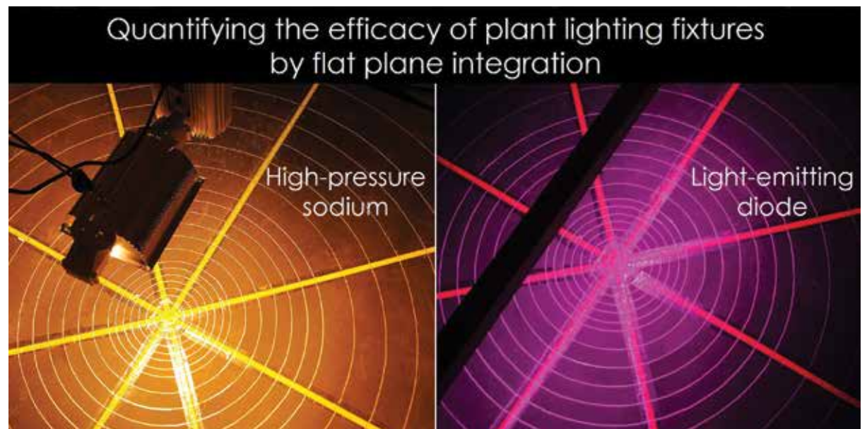
Figure 1. Two lamps being tested in a specialized room at Utah State University. (Photos: Jakob Johnson, Utah State University)
